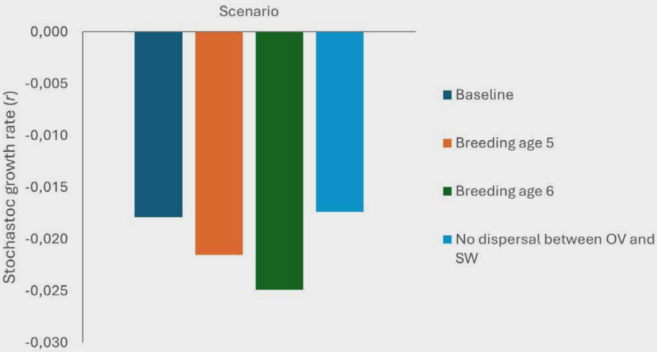
Figure 10: A plot indicating the stochastic growth rate of different model scenarios, comparing the baseline with models where age of first breeding in the metapopulation is 5 or 6 (rather than 4 as in the baseline) and models where there is no dispersal between the Overberg and Swartland (as opposed to 2-4% dispersal between these populations in the baseline).
